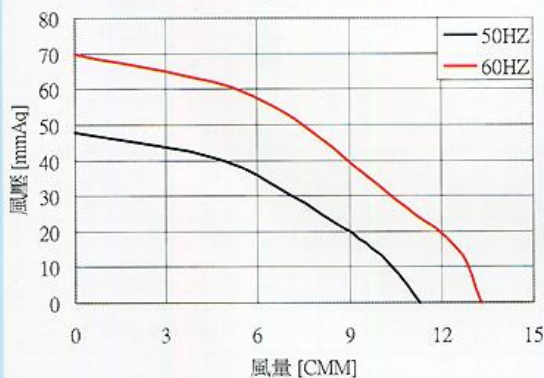
TBO-270505 [入口5"出口5"]
